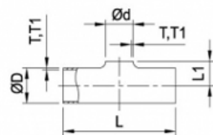
Welding Reducing Tee Without Straight-End
