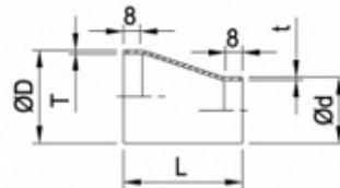
SMS Eccentric Reducer
