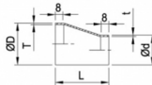
SMS ER SMS Eccentric Reducer
