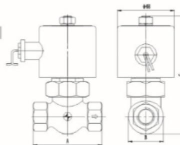
2L-series solenoid valve drawing
