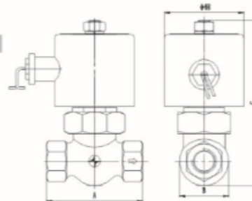
2L-series solenoid valve drawing
